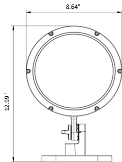
Base mounting
