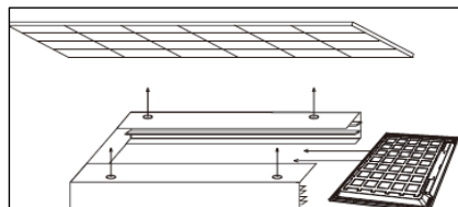
Surface Mount
