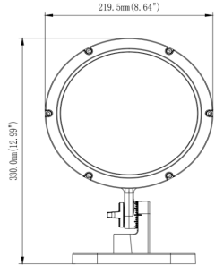
Base mounting
